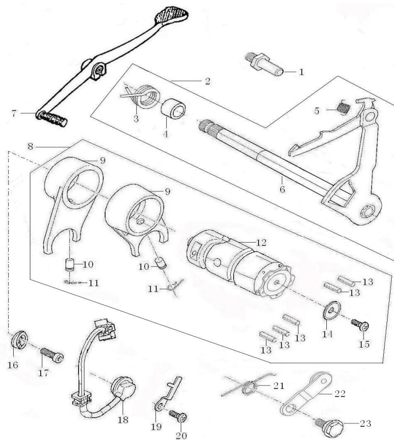
变速机构 GEARSHIFT MECHANISM
