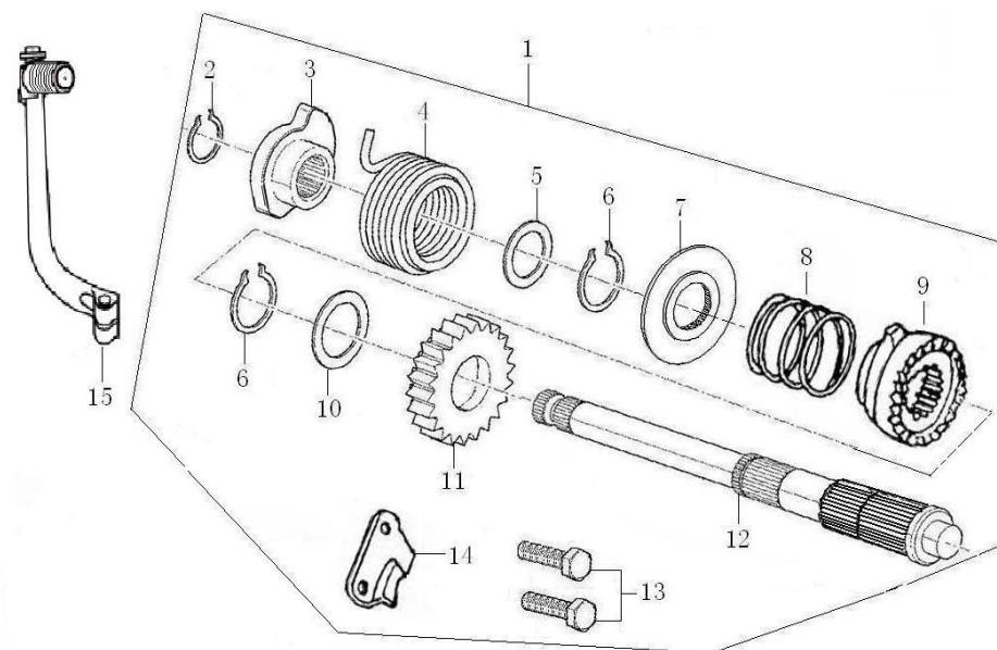
启动轴总成 KICK STARTING SHAFT ASSEMBLY
