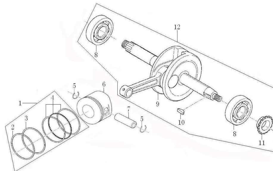
曲轴连杆部件/活塞 CRANKSHAFT CONNECTING-ROD ASSY/PISTON
